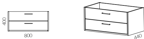
Wariant cabinet module - two drawers
