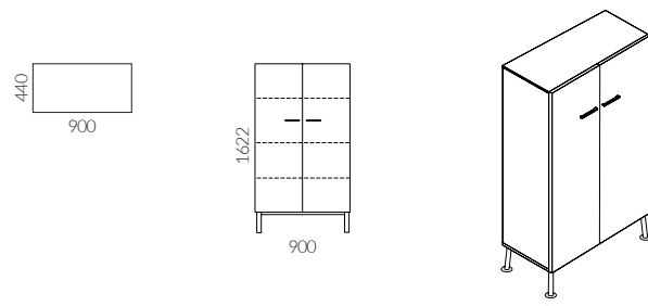
Sirio high cabinet
