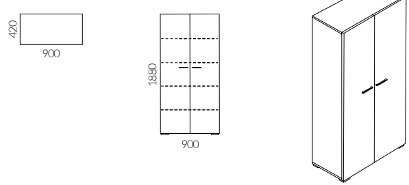
Sirio cabinet for documents
