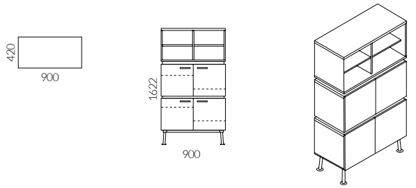
Sirio high cabinet
