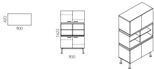
Sirio cabinet for documents and clothes
