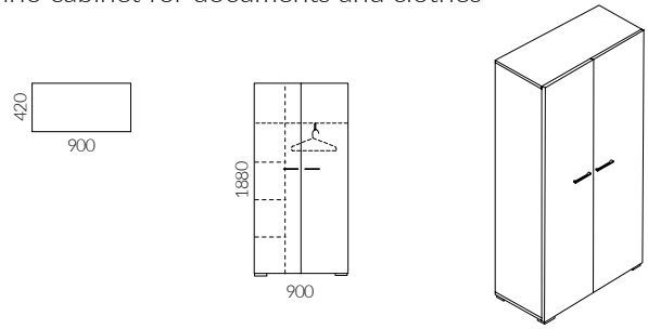
Sirio cabinet for documents and clothes
