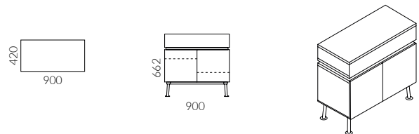
Sirio low cabinet with drawer
