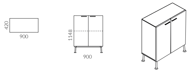
Sirio midle cabinet
