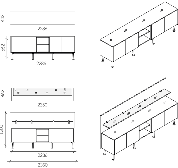
Sirio wide executive showcase with open segment
