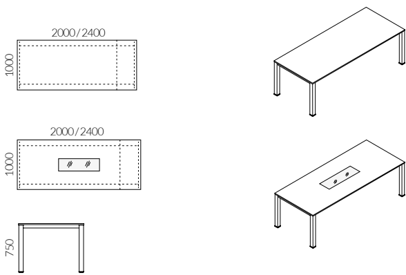
Graf rectangular conference table
