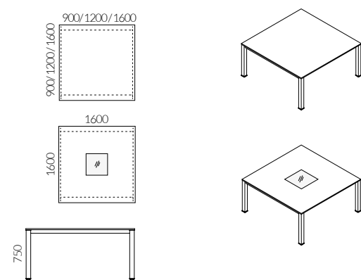
Graf square conference table
