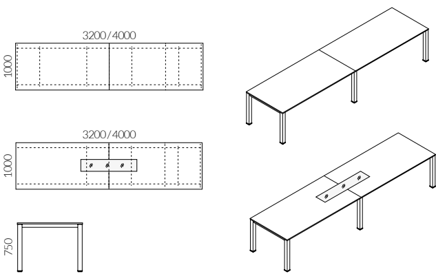
Graf conference table, rectangular two-piece top
