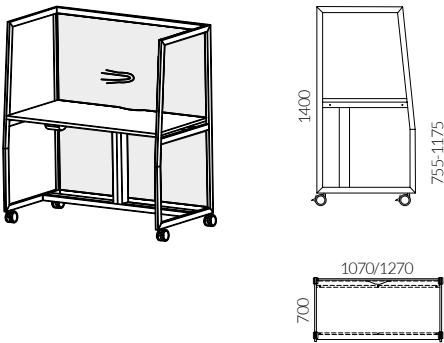
Desk with high partitions and pneumatic height adjustment - board wall
