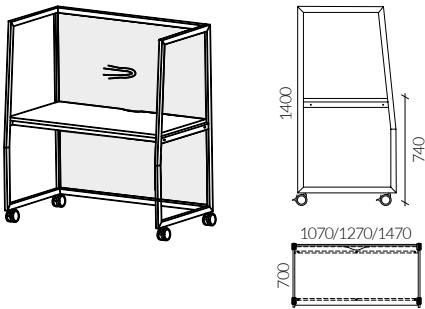
Desk with high partitions - board wall
