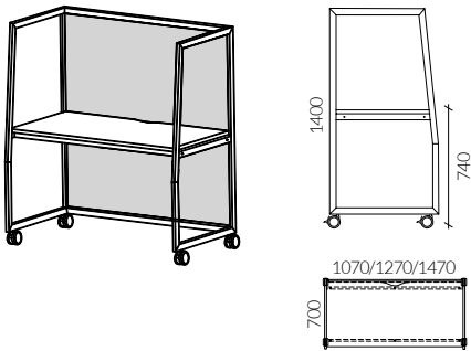
Desk with high partitions - upholstered wall from the inside
