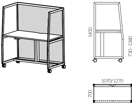
Desk with high partitions and electric height adjustment - upholstered panel from the inside
