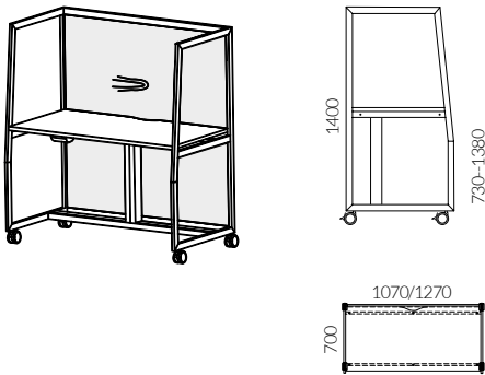
Desk with high partitions and electric height adjustment - board wall
