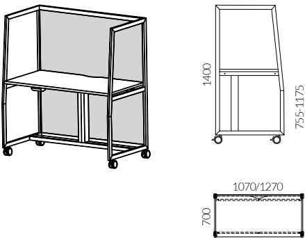
Desk with high partitions and pneumatic height adjustment - upholstered panel from the inside
